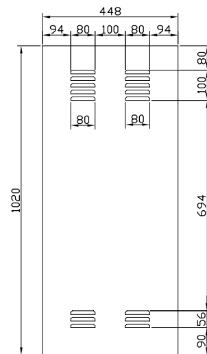
VISTA FRONTAL
